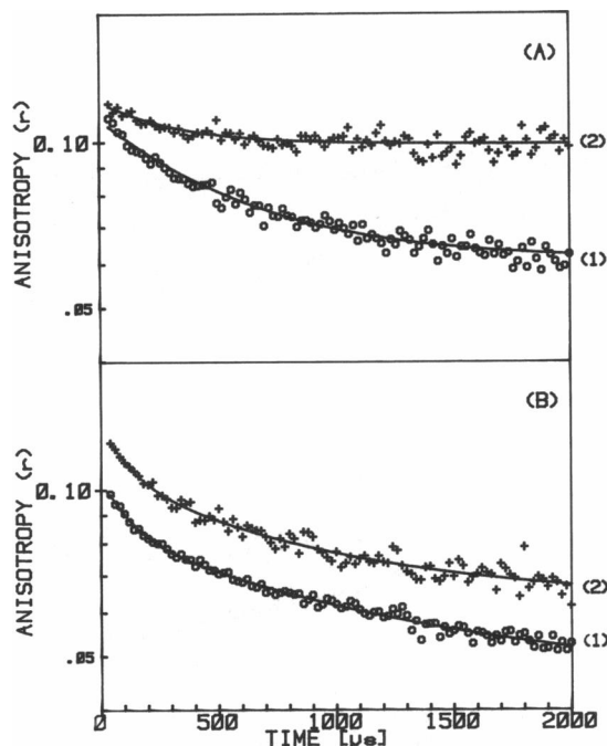
FIGURE 3 Effects of B6 and B10 on band 3 rotational mobility in ghosts. Samples contained 1.1 mg of membrane protein in 0.5 ml of 5PB; measurements were at 37°C. (A) (1), control; (2), 200 µg B6. (B) (1), control; (2), 400 µg B10. Note that curve 2 has been displaced upwards for clarity; otherwise it superimposes on curve 1.
