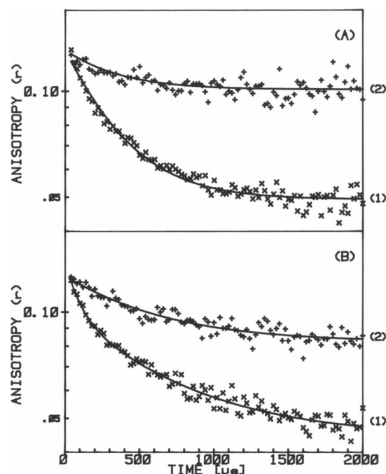
FIGURE 6 Effects of B6 and B17 on band 3 rotational mobility in stripped ghosts. Samples contained 0.5 mg of membrane protein in 0.5 ml of 5PB; measurements were at 37°C. (A) (1), control; (2), 200 µg B6. (B) (1), control; (2), 200 µg B17.
