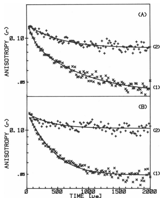
FIGURE 5 Effects of B14 and R18 on band 3 rotational mobility in stripped ghosts. Samples contained 0.5 mg of membrane protein in 0.5 ml of 5PB; measurements were at 37°C. (A) (1), control; (2), 200 µg R18. (B) (1), control; (2), 200 µg B14.
